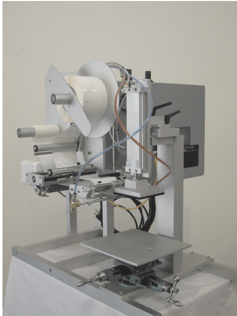
TAMP APPLICATOR
